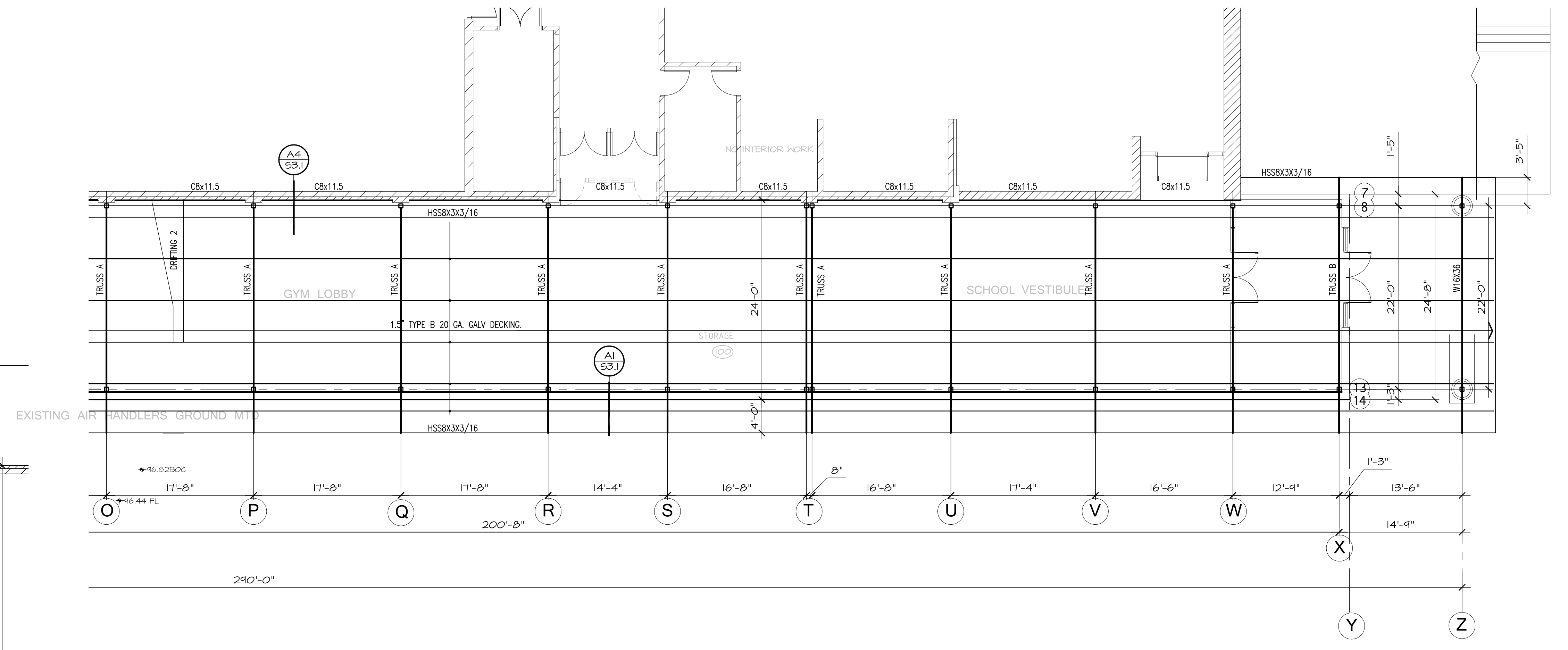
PARTIAL ROOF FRAMING 1/8" = 1'-0"
