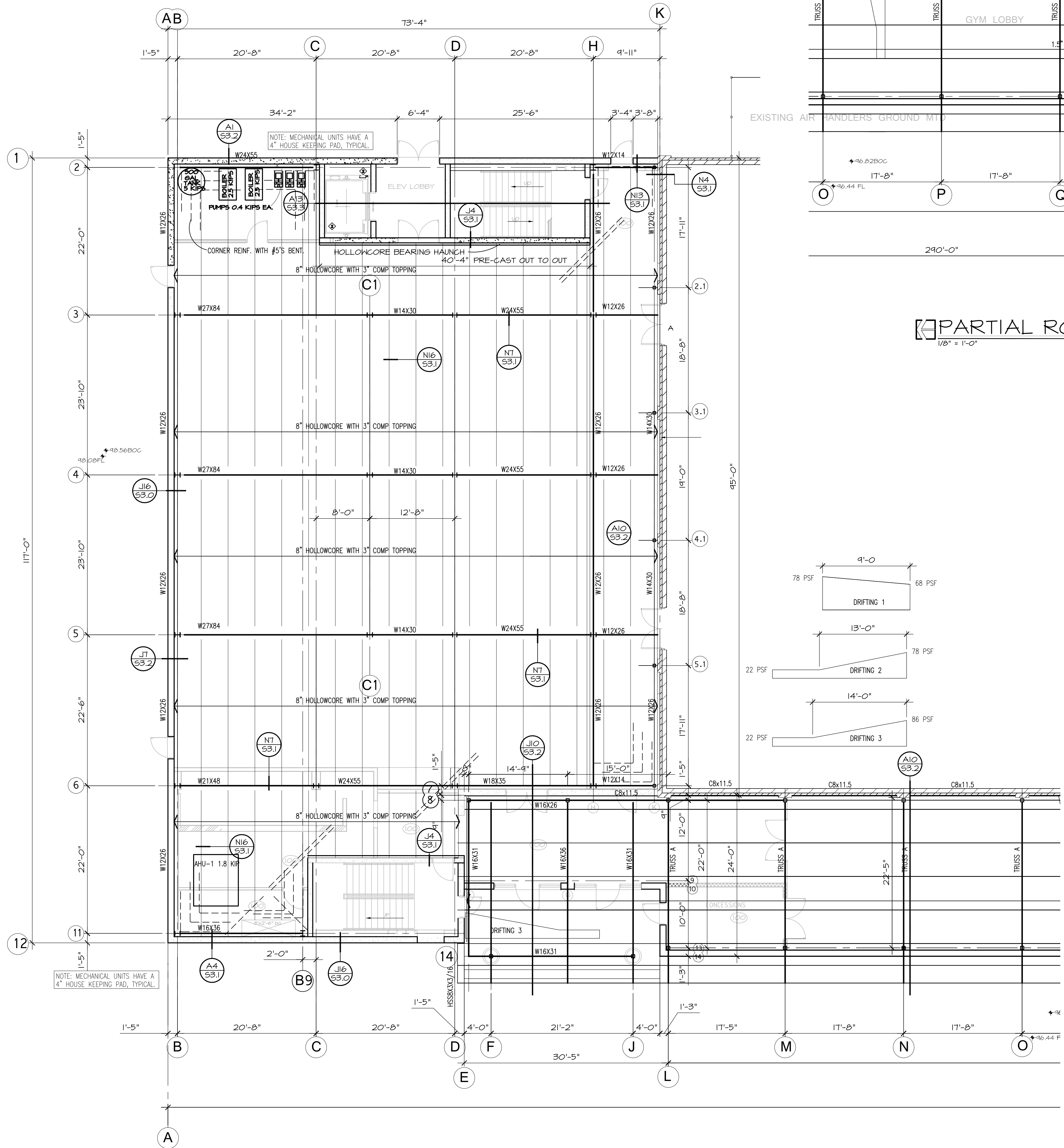
SECOND FLOOR FRAMING 1/8" = 1'-0" 105 THIS FLOOR 112-7
