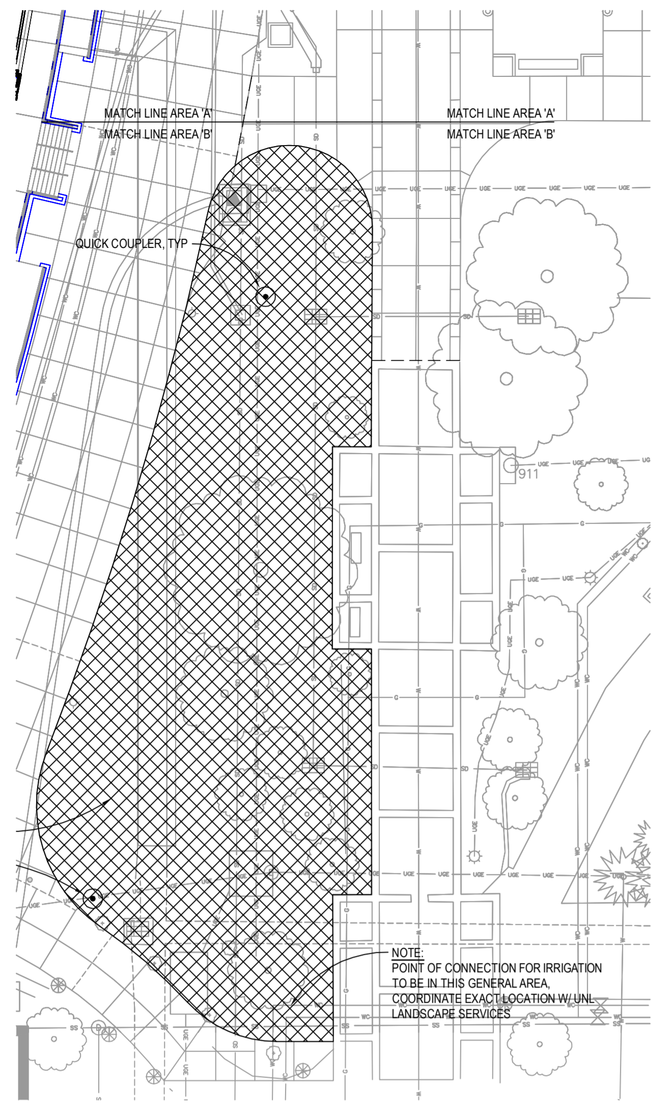
SITE IRRIGATION PLAN: AREA 'B' SCALE: 1"=20'-0"
