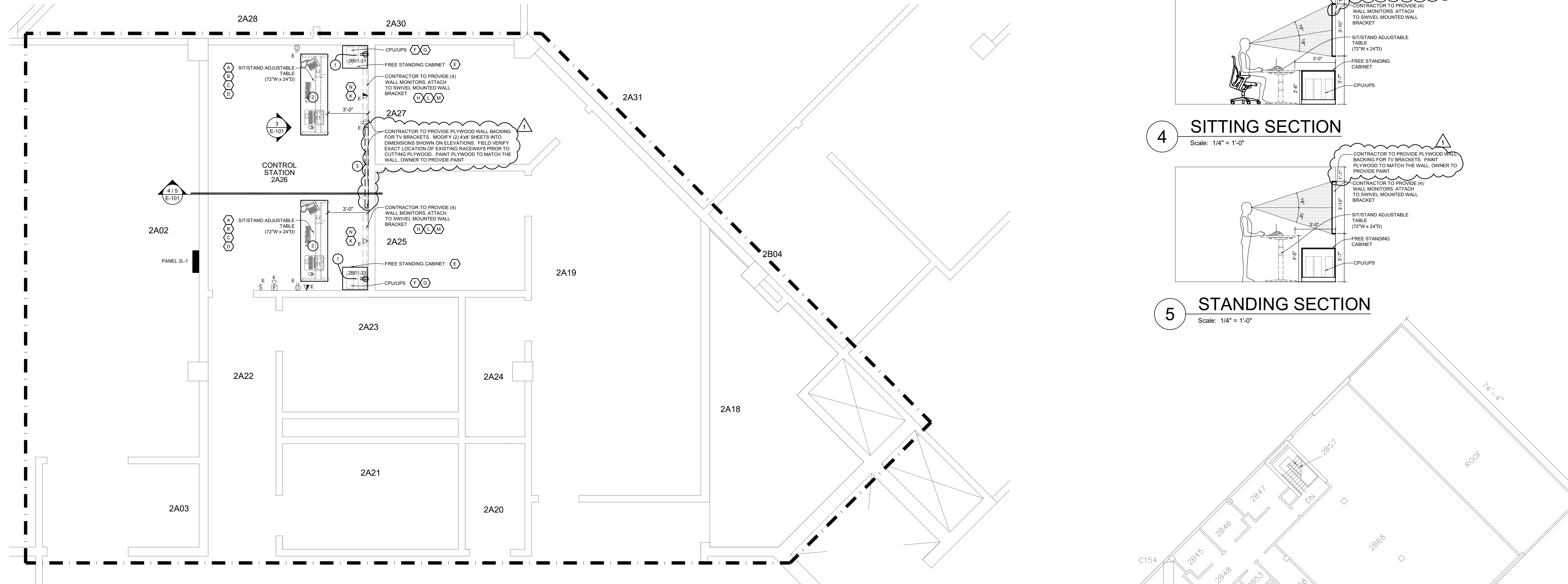
2 Enlarged Data Room Plan SCALE: 1/4" = 1'-0"
